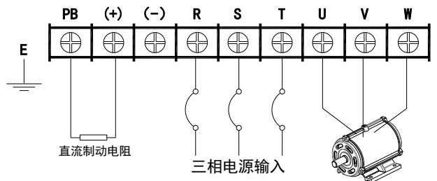
d) 37kW-45kW 变频器主回路端子排配线图
