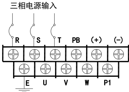
i) 280kW-450kW 变频器主回路端子排配线图
